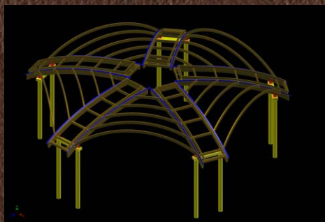
100' Diameter Dome conceptual drawing.
